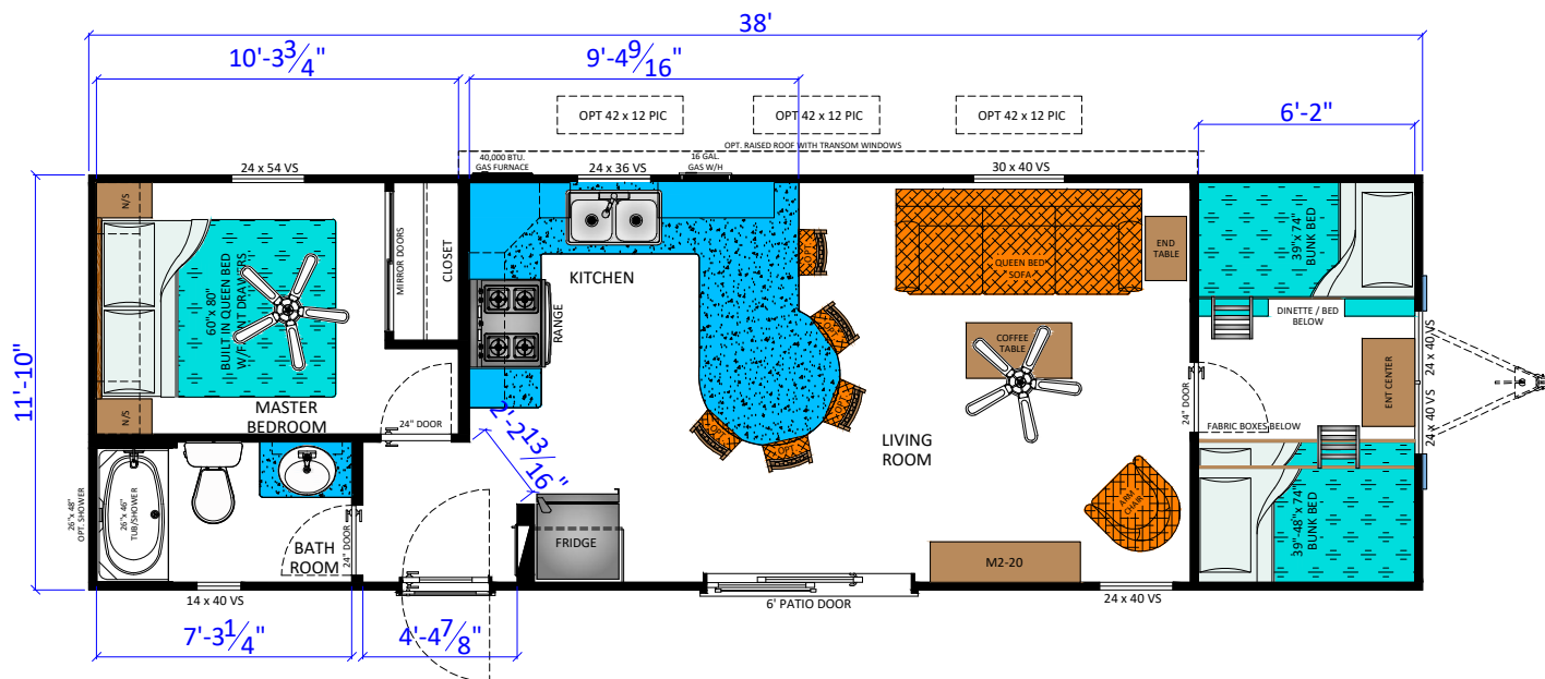
FREEDOM 21-2 (F3812 2BR) (450 SQ.FT.) PARKBRIDGE Stock
