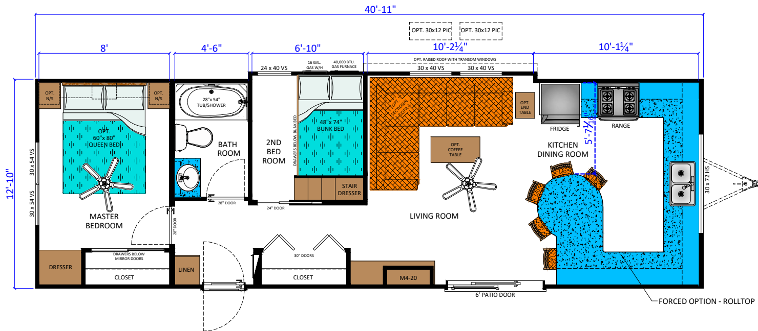
MINNISET 21 (4113 2BR FK) (537 SQ.FT.) PARKBRIDGE Stock
