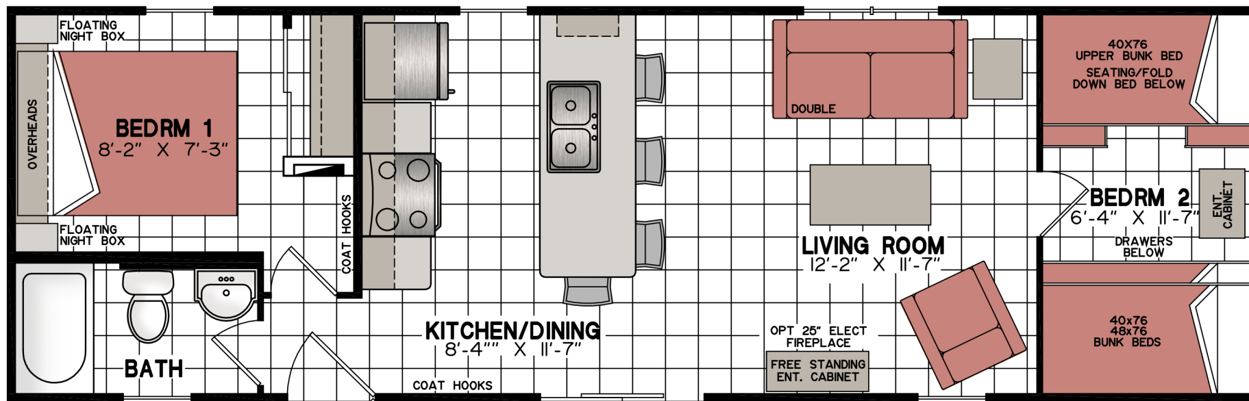
20-4954-2 38' x 12' Reflection (456sq.ft.)
